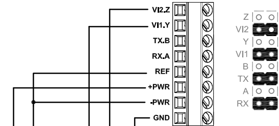
Output Jumper J1 Configuration
