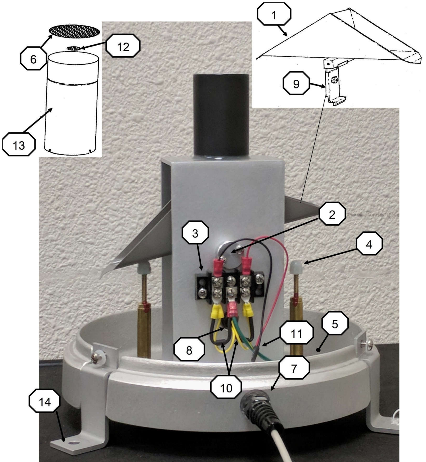
Figure 6-2 370D Parts
