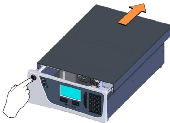
Figure 25 – Opening the Instrument – 3
