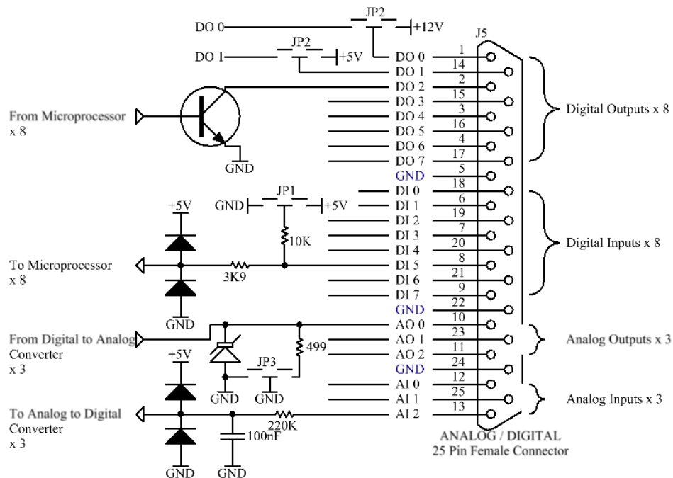
Figure 86 – Analog & Digital I/O Individual Pin Descriptions
