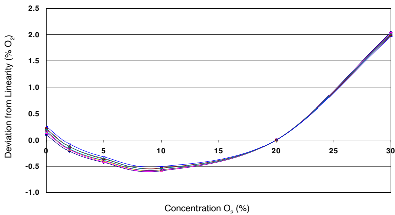
Figure 3 Linearity
