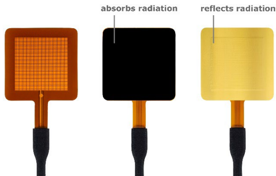
Figure 3 example: FHF05-50X50 foil heat flux sensor without and with BLK-50X50 and GLD-50X50 stickers applied to it
