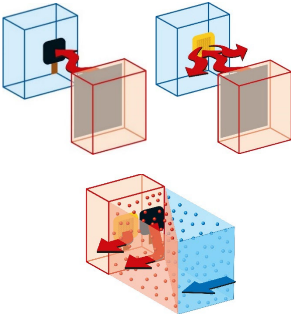
Figure 4 the working principle of BLK – GLD stickers: sensors equipped with black absorbing stickers will absorb all radiation while gold reflective stickers reflect all radiation. Both stickers are sensitive to convective heat flux
