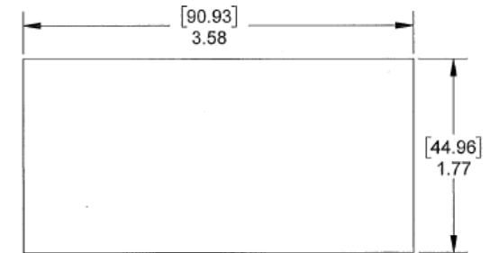
PANEL CUTOUT
