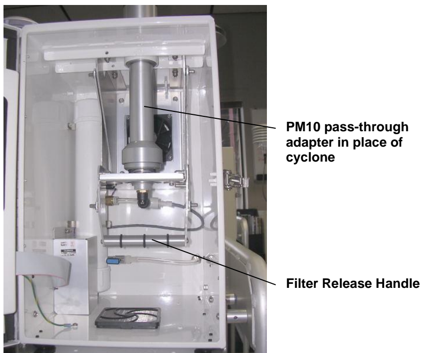
Figure 2-7 PM 10 Configuration
