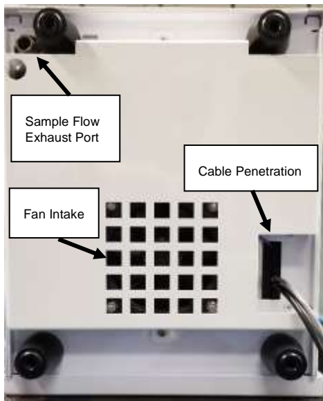
Figure 3-10 Bottom of E-FRM-DC Enclosure
