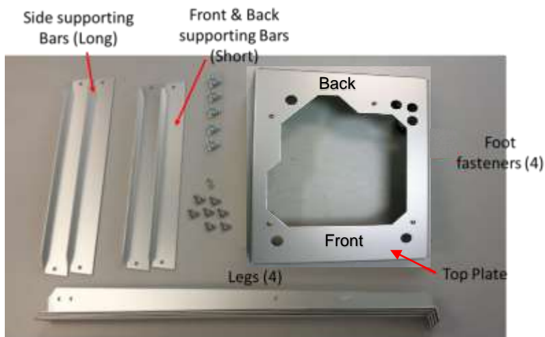
Figure 3-2 E-FRM-DC Sampler Stand Components
