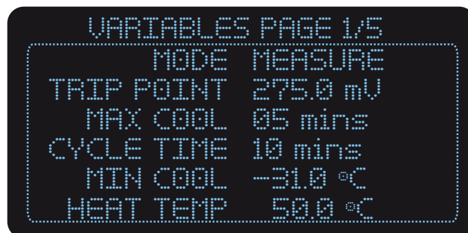
Figure 23 Variables Page
