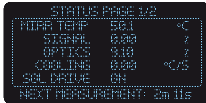
Figure 17 STATUS Page 1
