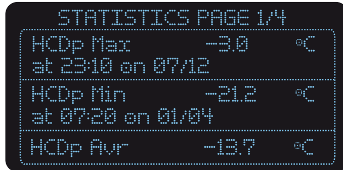
Figure 20 STATISTICS Page
