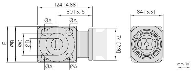
WFC Flange Wafer Flow Cell
