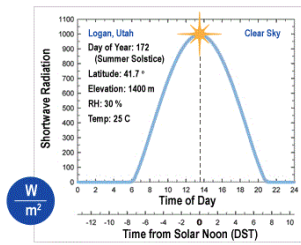
MODEL FOR PYRANOMETER SHORTWAVE RADIATION
