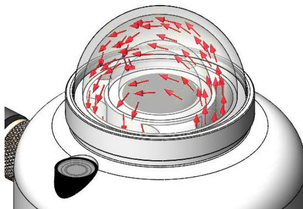
Figure 4 how it's done: recirculating ventilation and heating between the inner- and outer dome is much more power efficient than traditional ventilation systems
