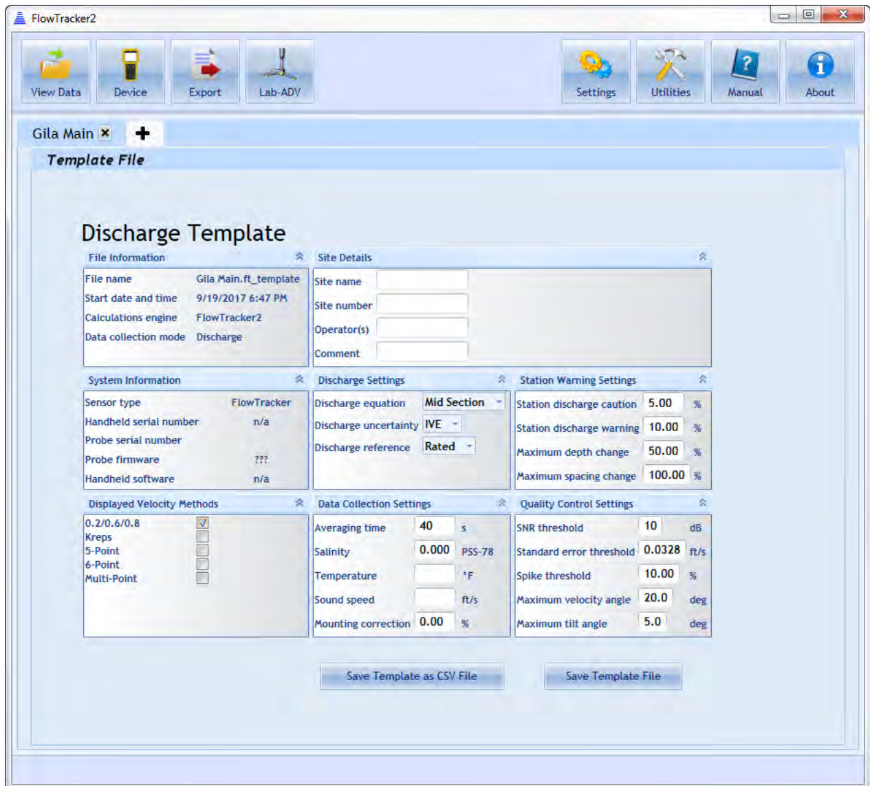
Figure 14:23 - Discharge Template
