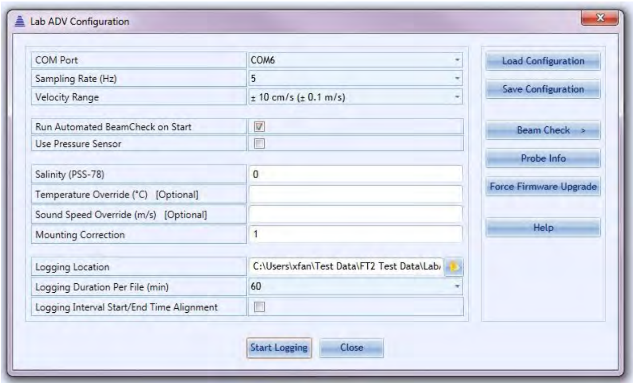
Figure 15:3 - Lab-ADV Configuration
