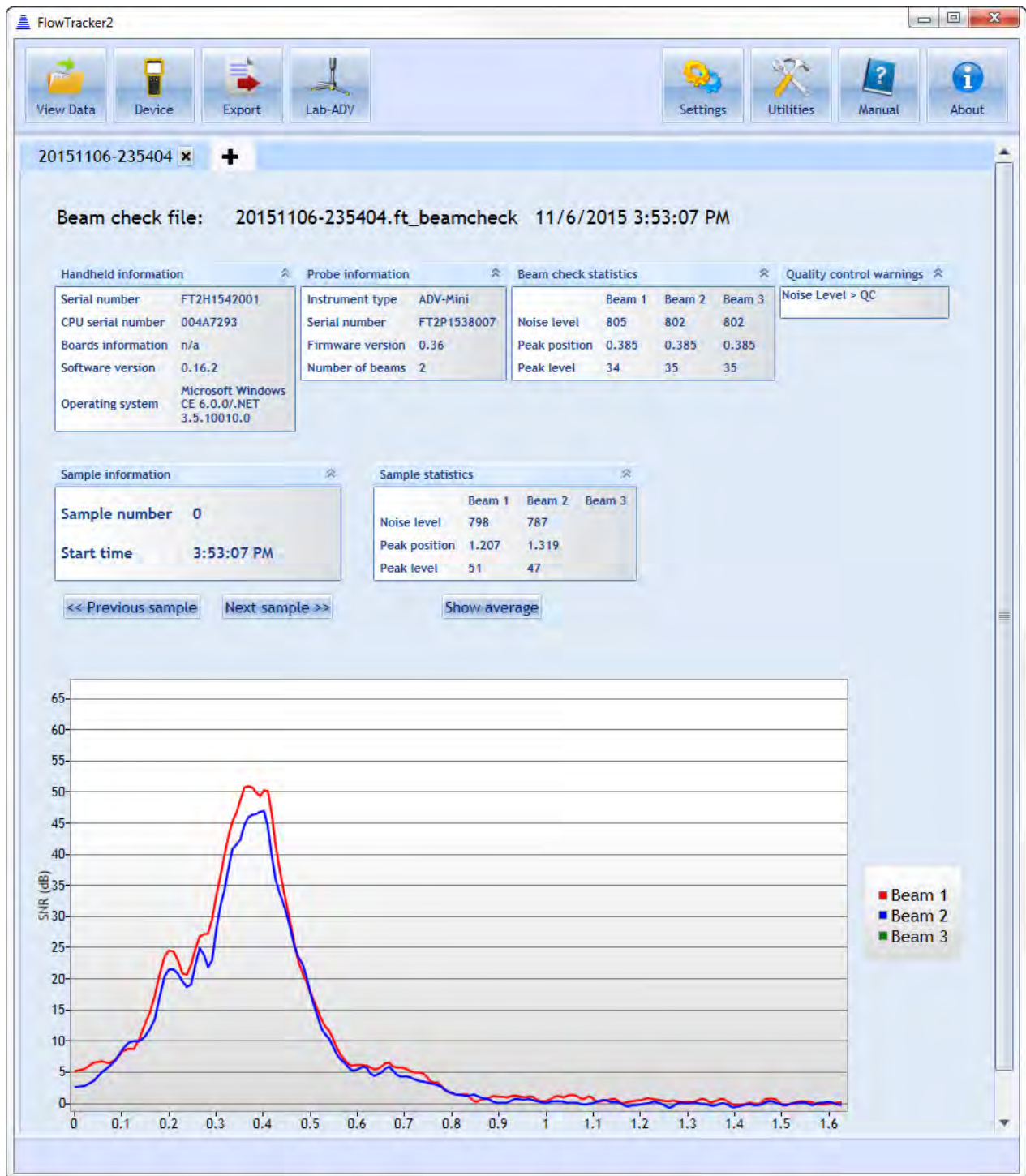
Figure 14:22. Viewing a Beamcheck File
