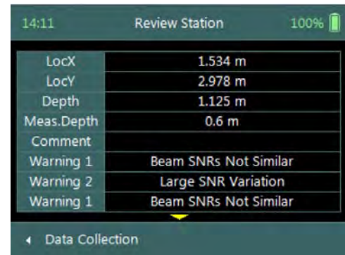
Figure 9:25 - Review Station
